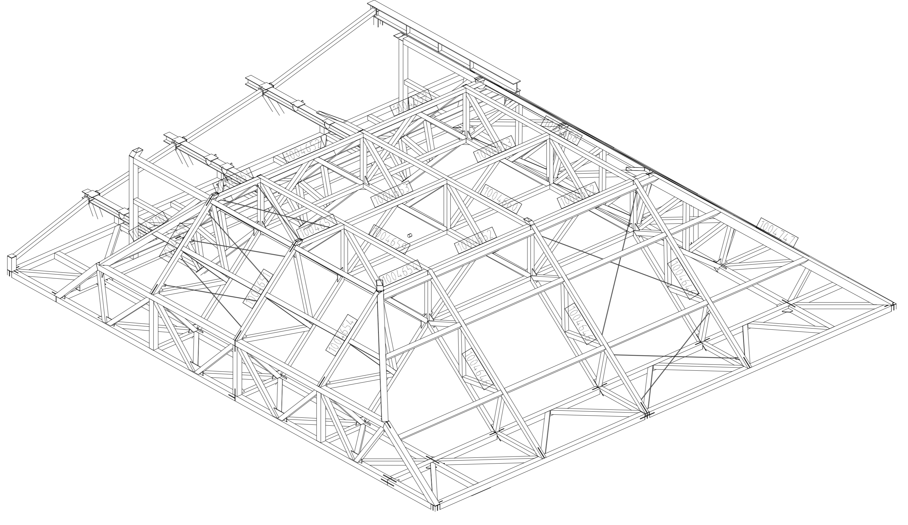
PARTIAL AXONOMETRY 2 / 3 1/75
