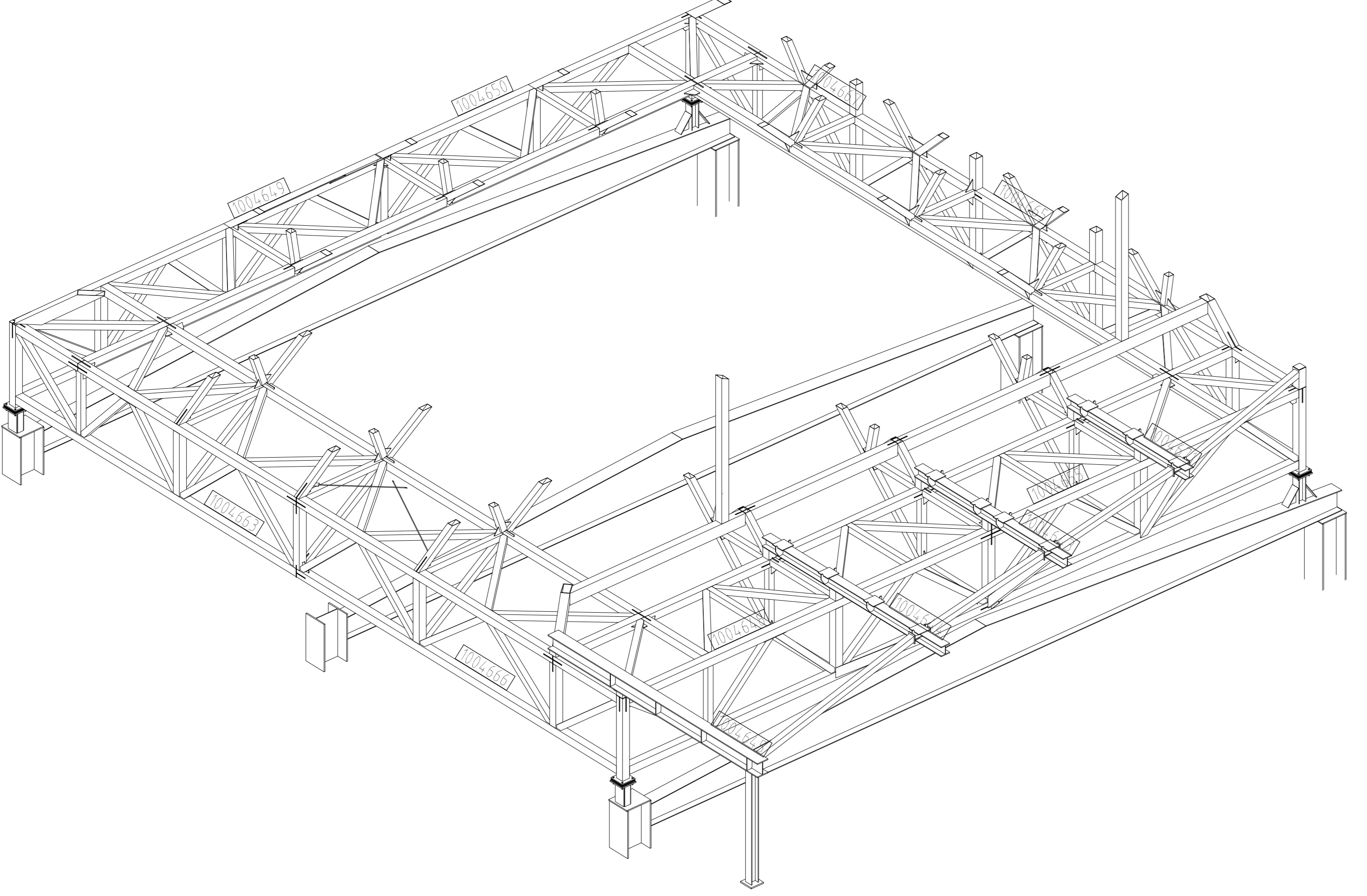
PARTIAL AXONOMETRY 1 / 3 1/75
