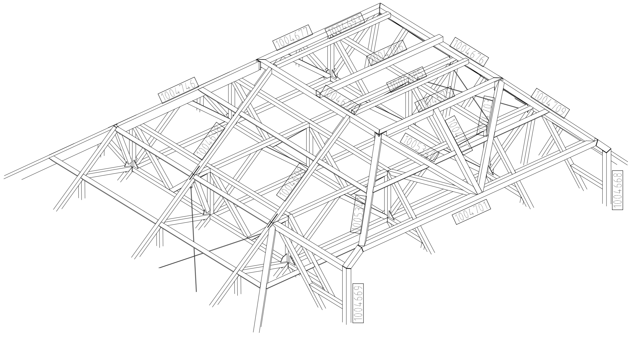
PARTIAL AXONOMETRY 3 / 3 1/75
