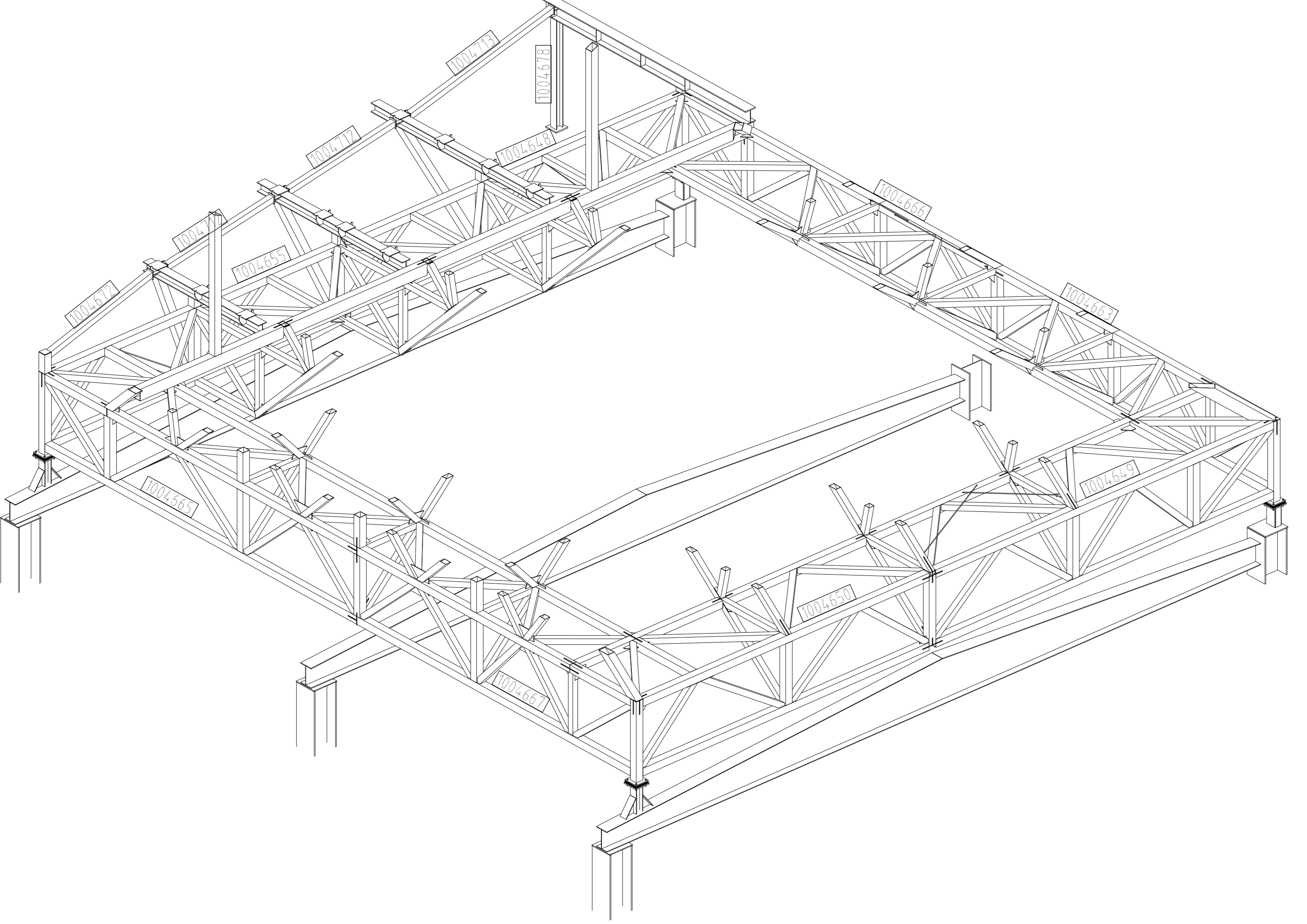
PARTIAL AXONOMETRY 1 / 3 1/75
