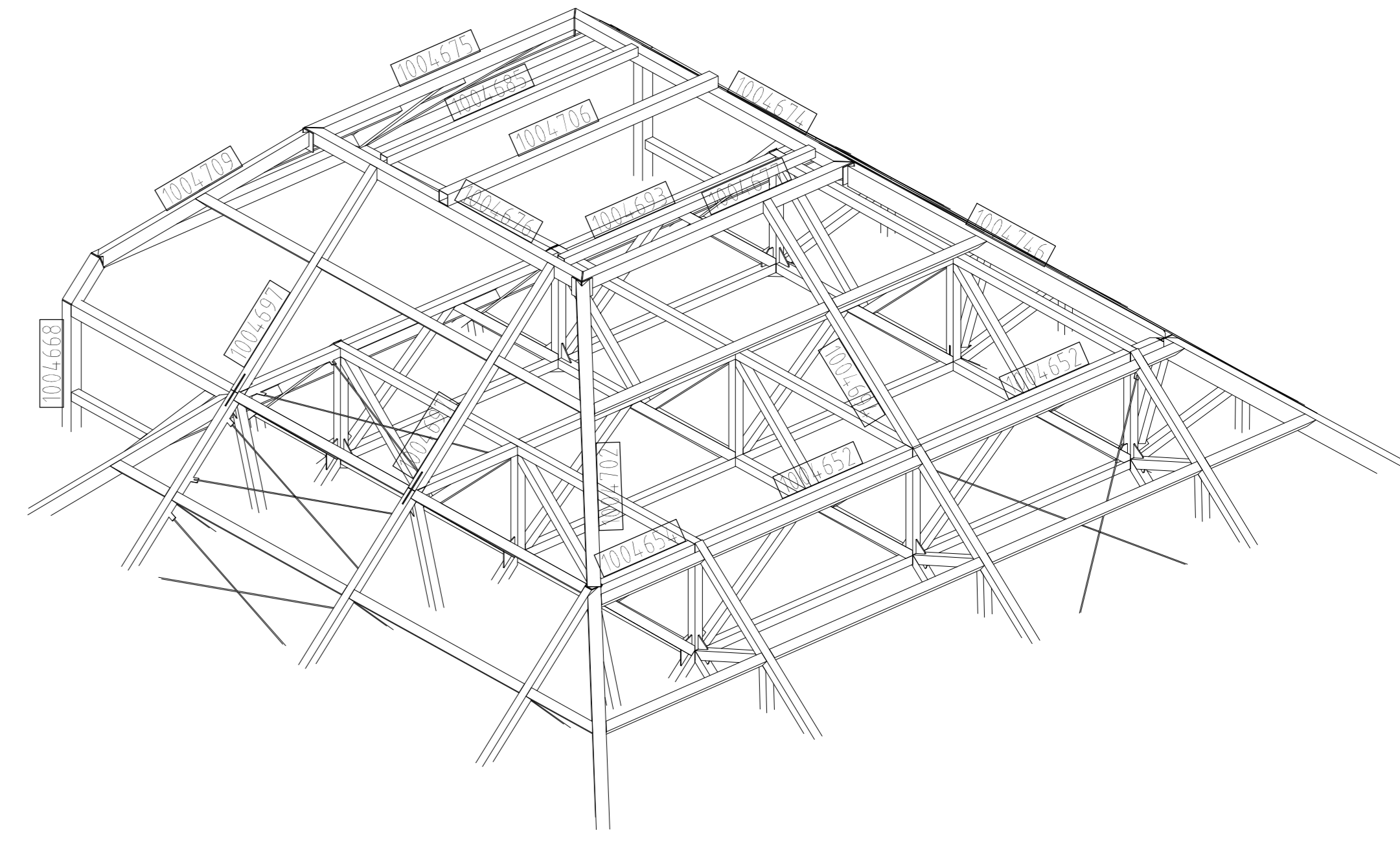
PARTIAL AXONOMETRY 3 / 3 1/75
