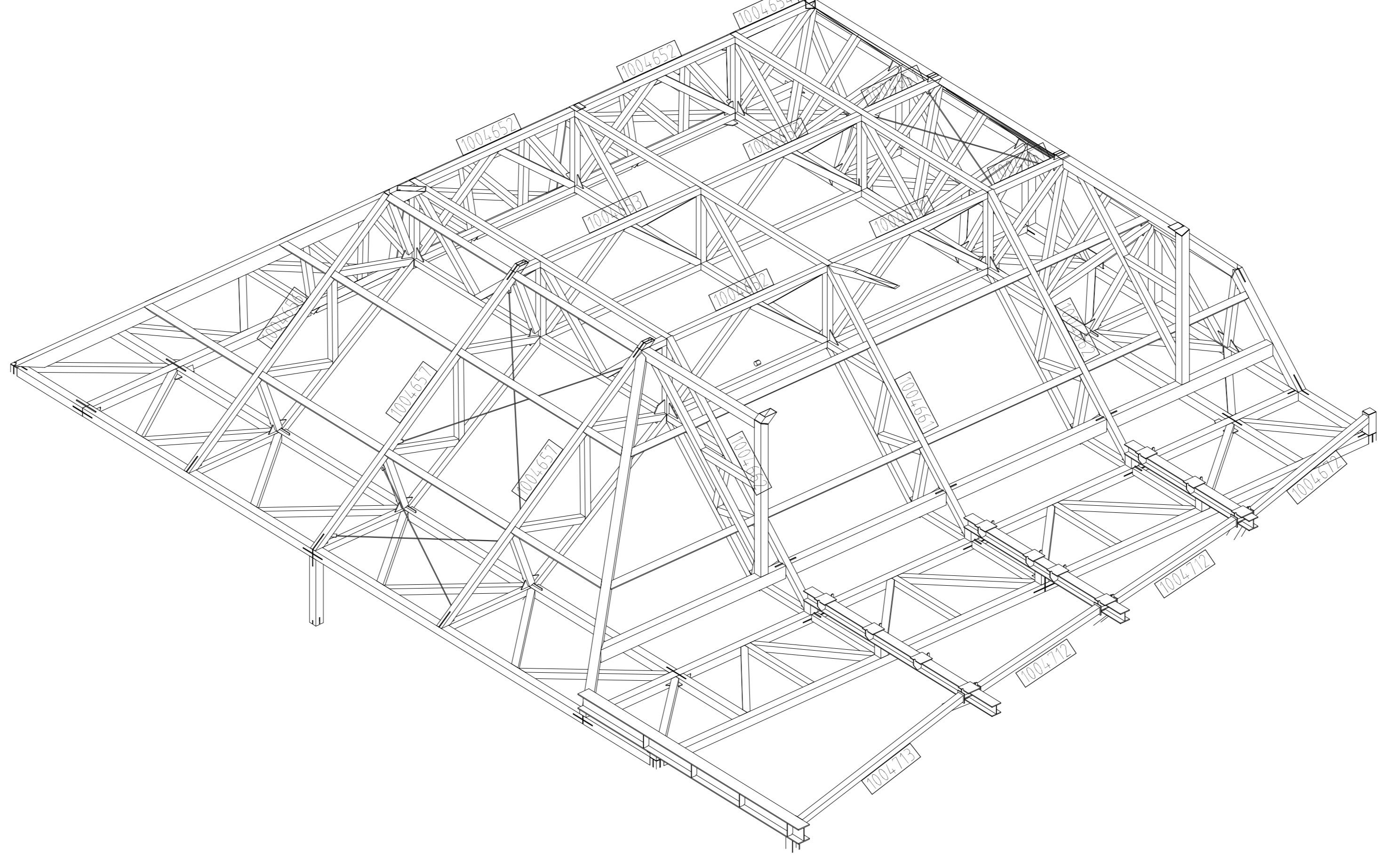
PARTIAL AXONOMETRY 2 / 3 1/75
